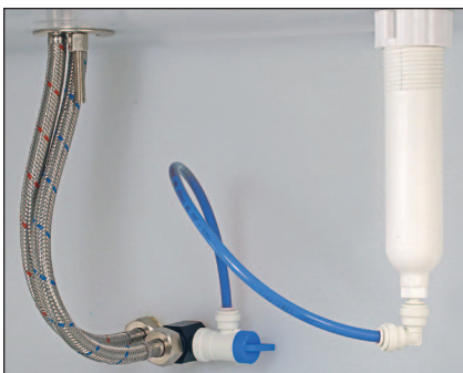
The All-In-One Clean Water Kit includes parts and instructions making installation easy.
